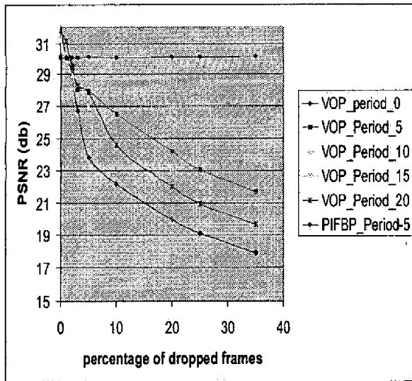
Figure 2 Performance under loss of Inter / Intra frame coding (Data rate = 128 kbps, fps =15 fps)
