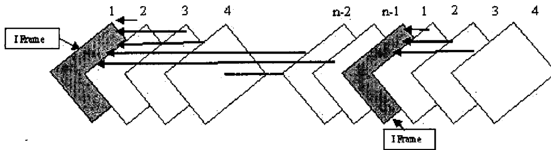
Figure 1 Periodic Intra frame based prediction (PIFBP)
